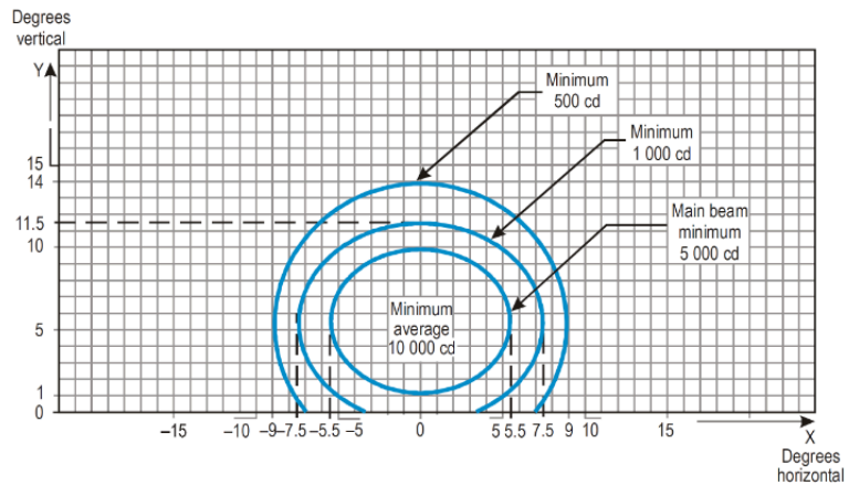
ICAO requirements Annex 14 Vol.1 Fig. A2-3.
