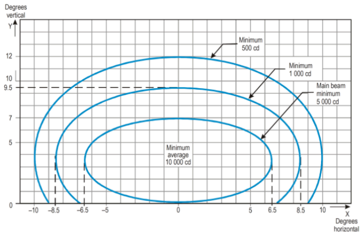
ICAO requirements Annex 14 Vol. 1 Fig. A2-10. White
