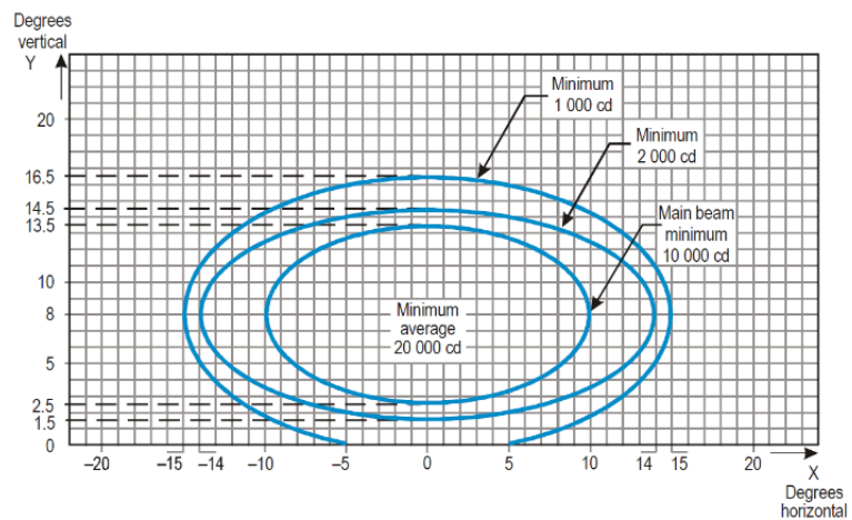
ICAO requirements Annex 14 Vol.1 Fig. A2-1.
