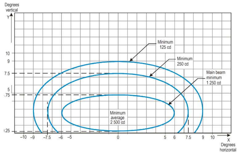
ICAO requirements Annex 14 Vol.1 Fig. A2-8.
