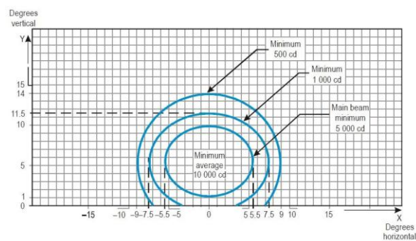
Low intensity: 10% Average 1000 cd Medium intensity: 30% Average 3000 cd
