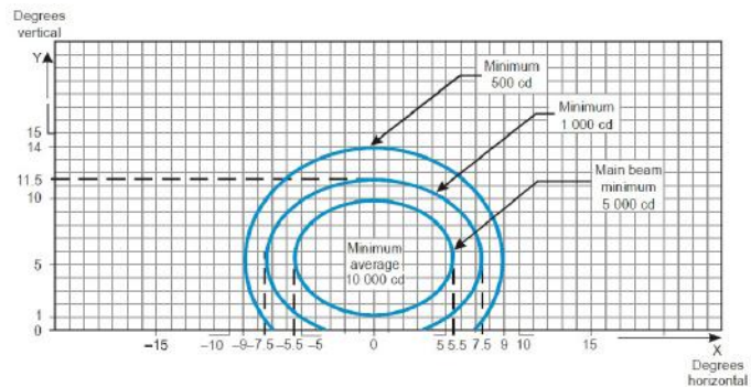
ICAO requirements Annex 14 Vol.1 Fig. A2-3. GREEN
