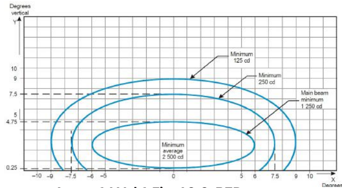
ICAO requirements Annex 14 Vol.1 Fig. A2-8. RED
