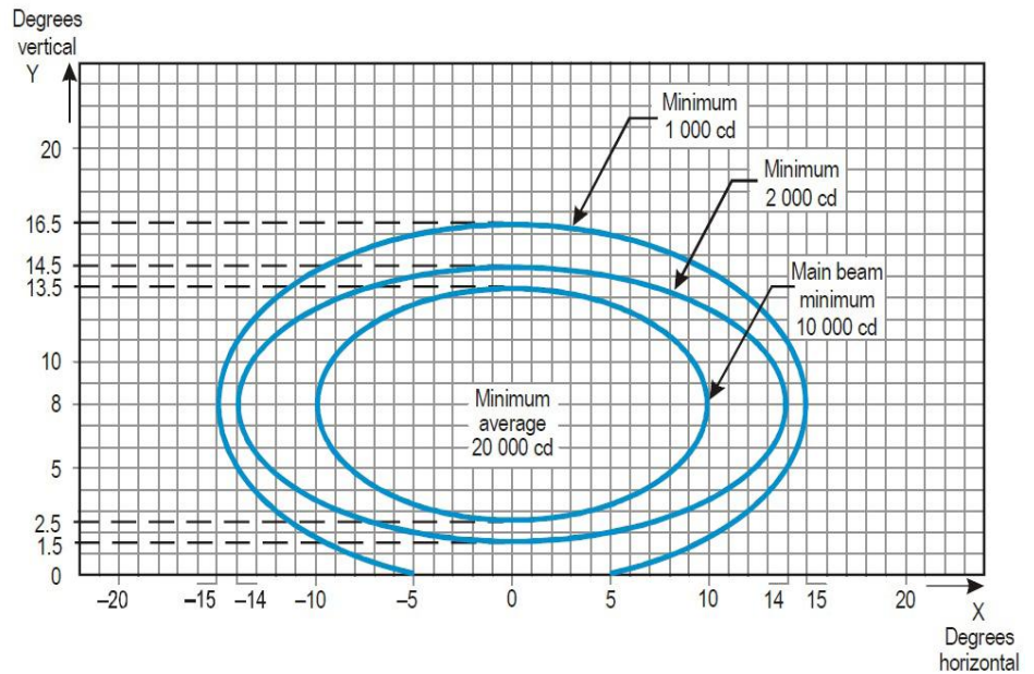
ICAO requirements Annex 14 Vol.1 Fig. A2-1.
